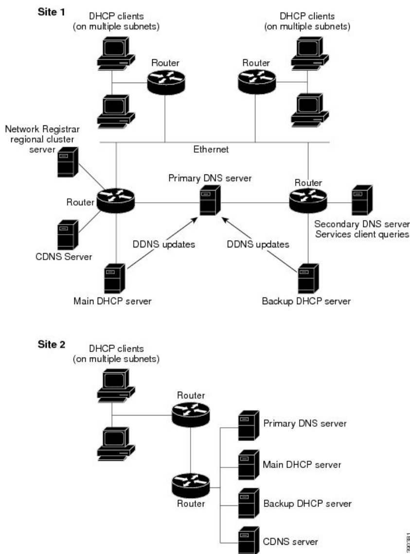
Figure 3: Large Enterprise or Service Provider Network Configuration
